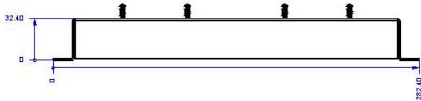
Figure 5: 208-0066 Surface Mounting Plate Dimensions
