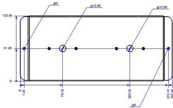
Figure 4 208-0066 Combined Surface mount
