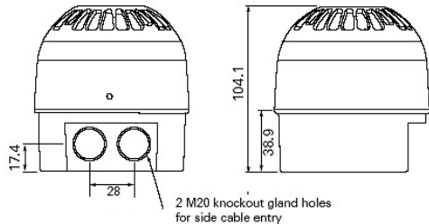
Figure 7: 208-0064 IP65 Deep Base Dimensions
