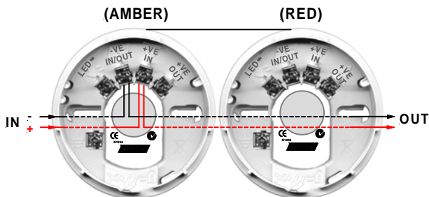
Figure 1: 208-0063 Combined Strobe Wiring
