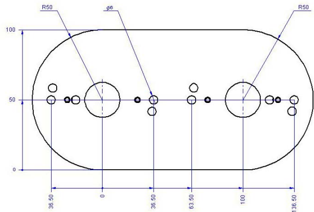
Figure 3: 208-0063 Flush Mounting Plate Dimensions
