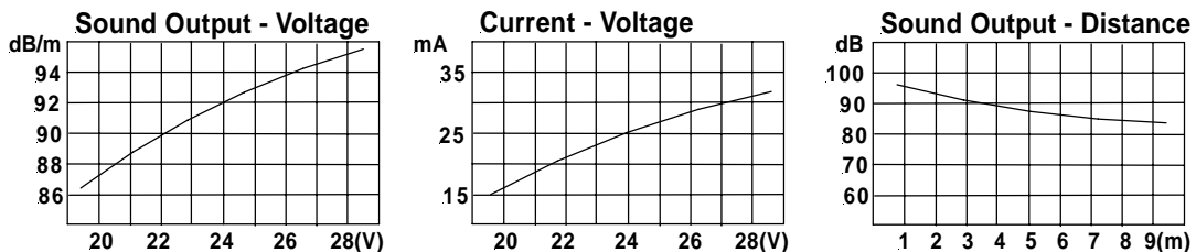
Performance Graphs of Ampac 150mm Fire Alarm Bell
