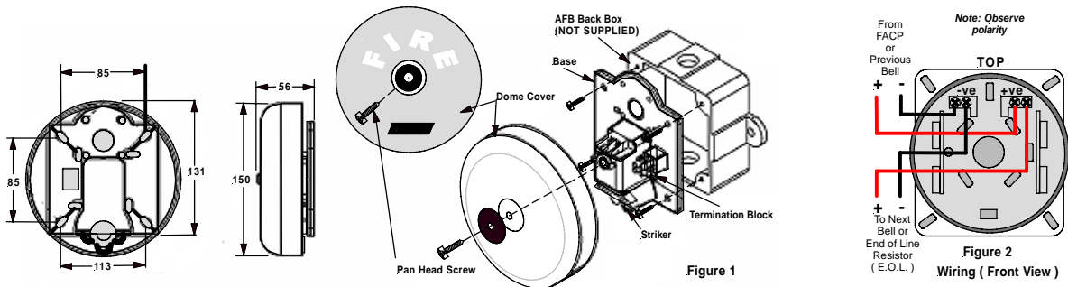
Installation of Ampac 150mm Fire Alarm Bell
