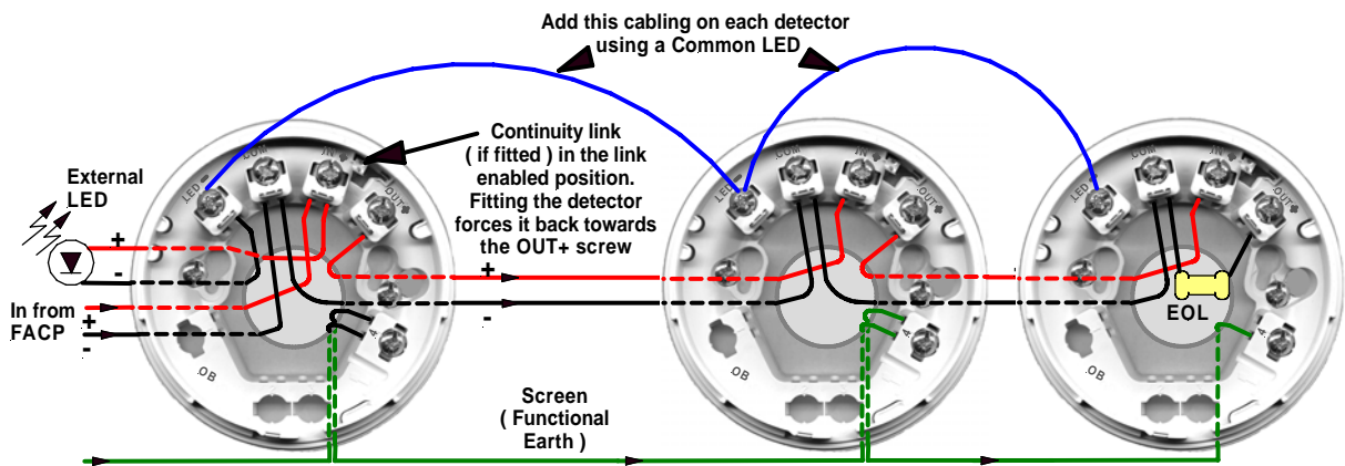
Figure 5: Base Wiring Diagram
