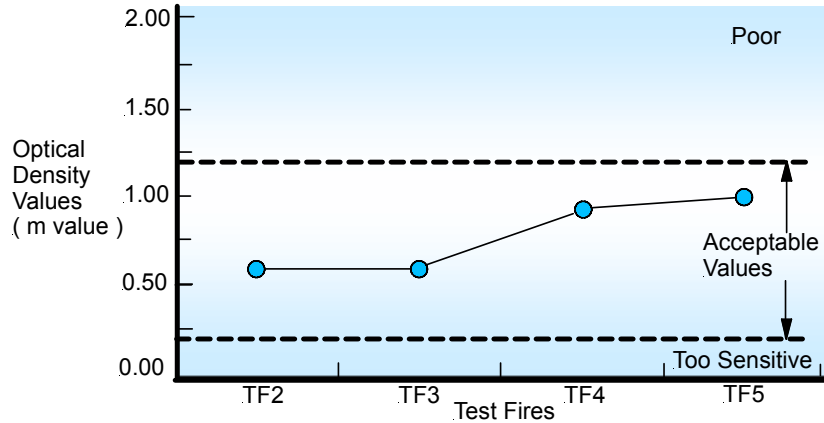
Figure 1: Orbis Optical Detector Response to Test Fires
