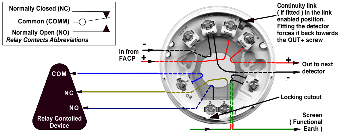
Figure 7: TimeSaver Relay Base Wiring Connections
