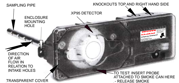
Figure 1: Duct Sampling Unit
