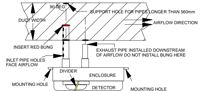
Figure 2: Detector Duct Installation
